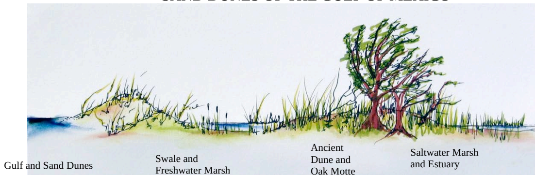
CROSS SECTION OF DUNE / SWALE COMPLEX OF GULF COAST
